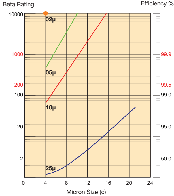
DFO-512... Efficiency
